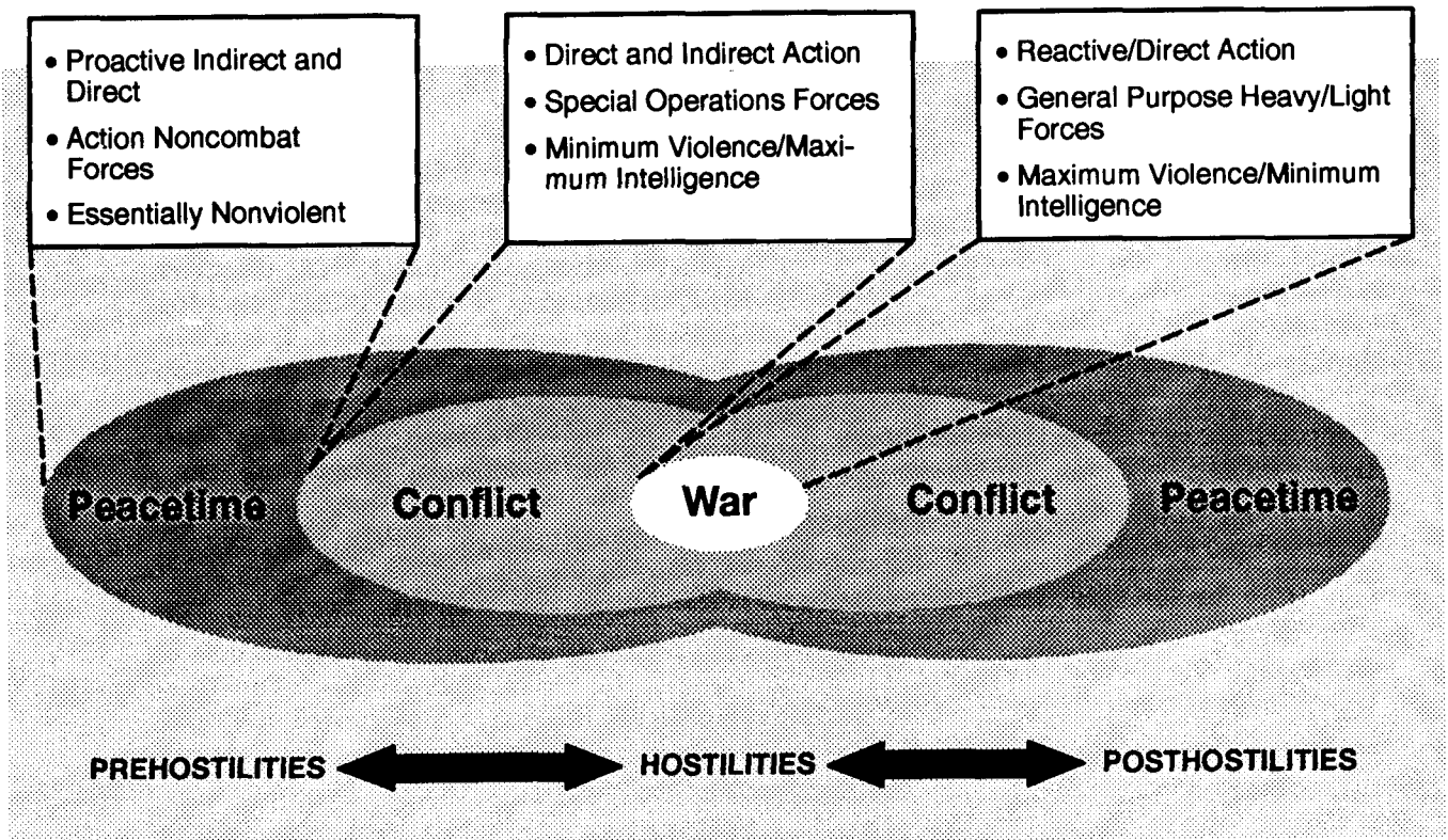
Figure 3-3. Operational continuum.
