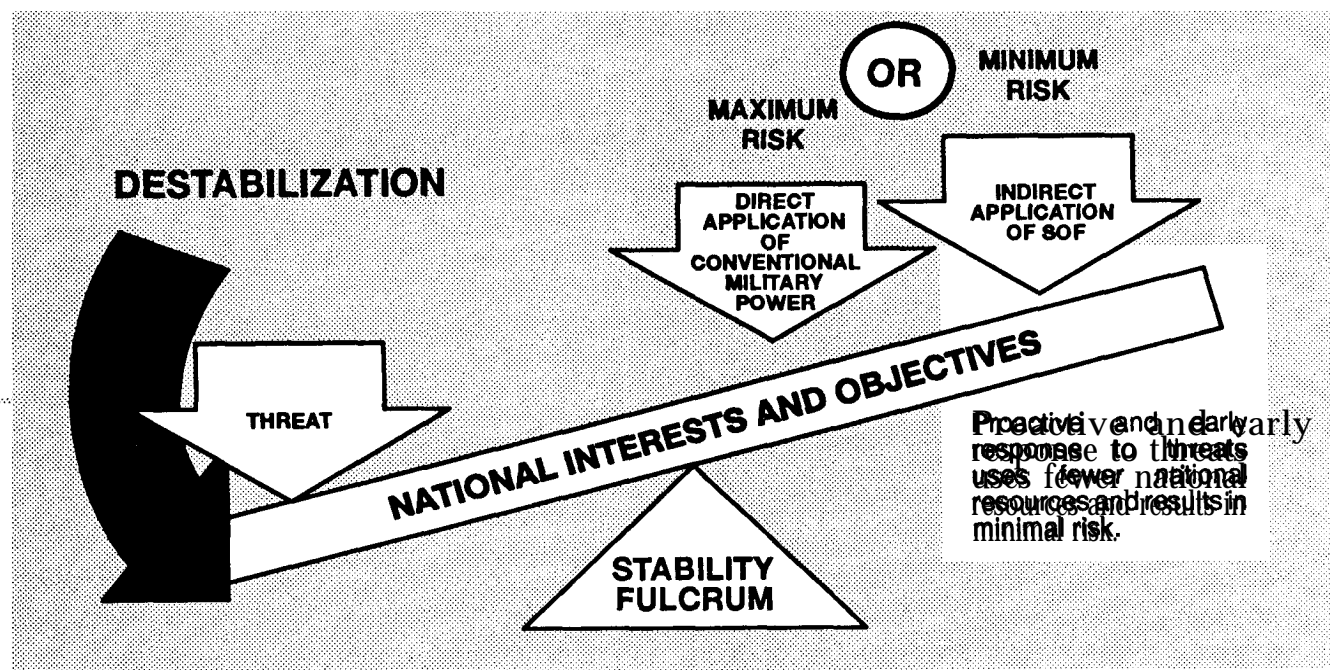
Figure 1-2. National response.
